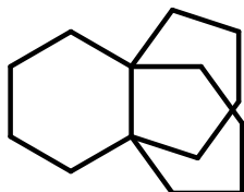
[4.4.4]propellane
